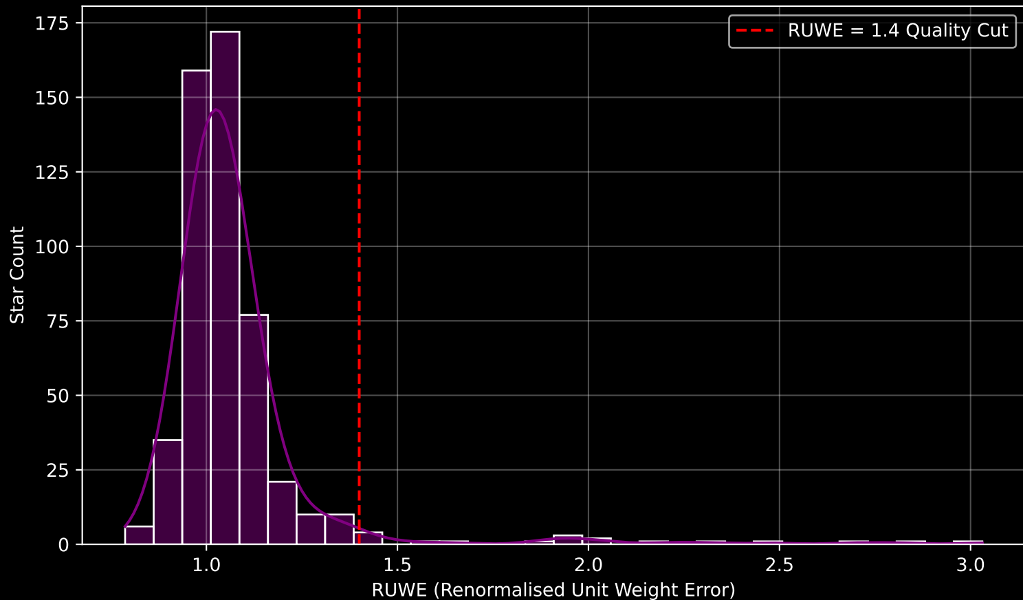
GAPOGEE DR17 Field [210+08] RUWE Distribution (n= 508)
