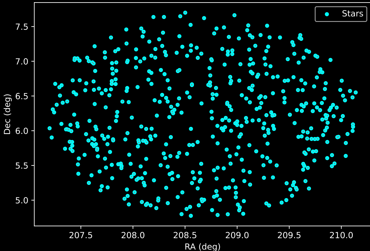
APOGEE DR17 Field: [210+08] Proper Motion Vectors for Gaia Star Field (n= 512)
