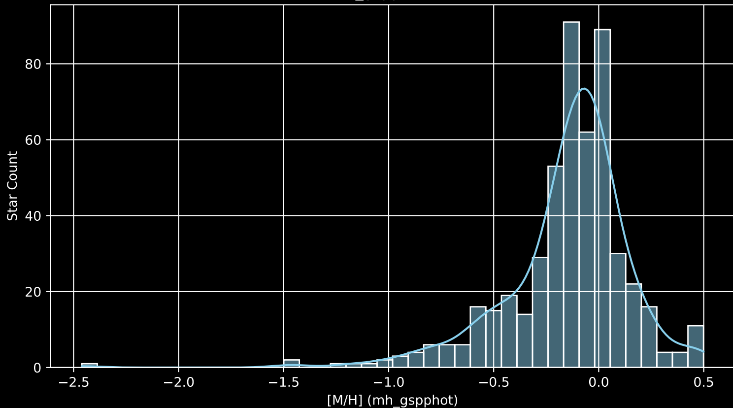
APOGEE DR17 Field: [210+08 [M/H] (mh_gspphot) (n= 508)
