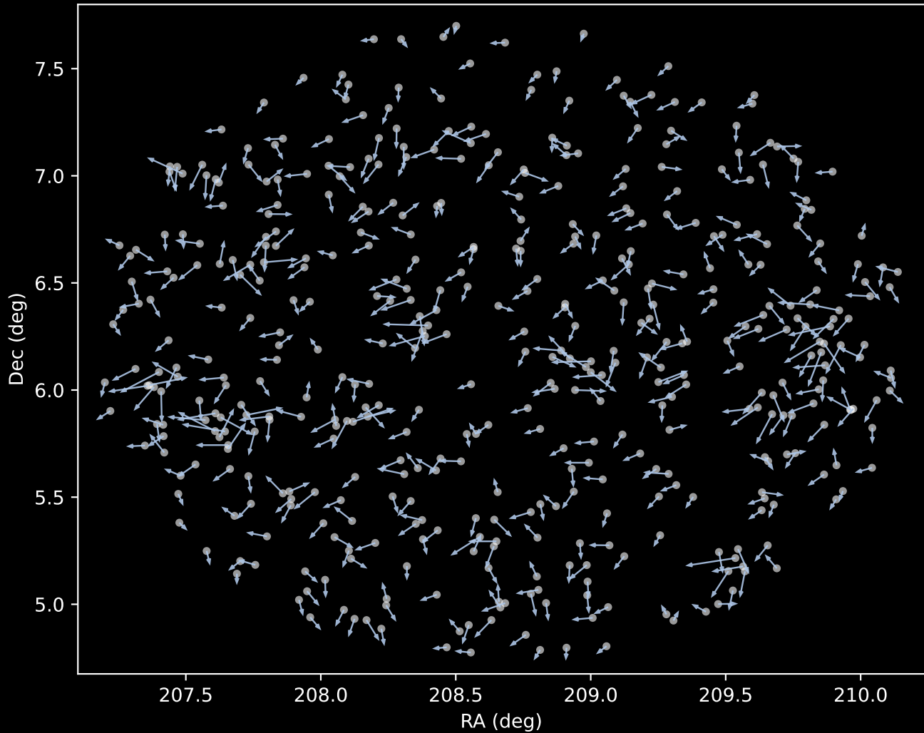
APOGEE DR17 Cluster 1 Proper Motion Vectors (n=463)
