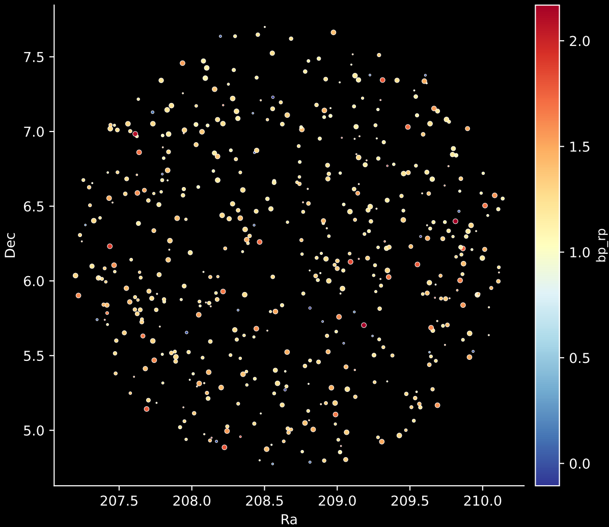
APOGEE DR17 Field: [210+08] Stars: 512
