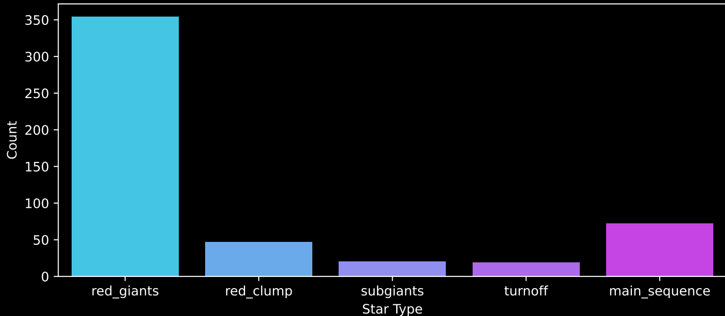
APOGEE DR17 Field: [210+08] Count plot of Star Type
