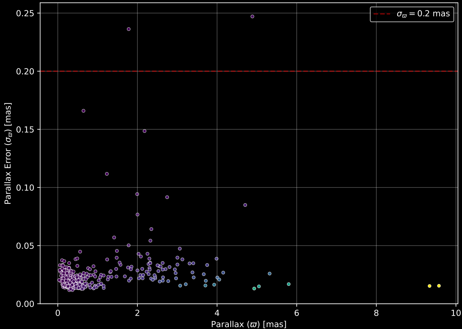
APOGEE DR17 Field: [210+08] Parallax Quality (n= 512)
