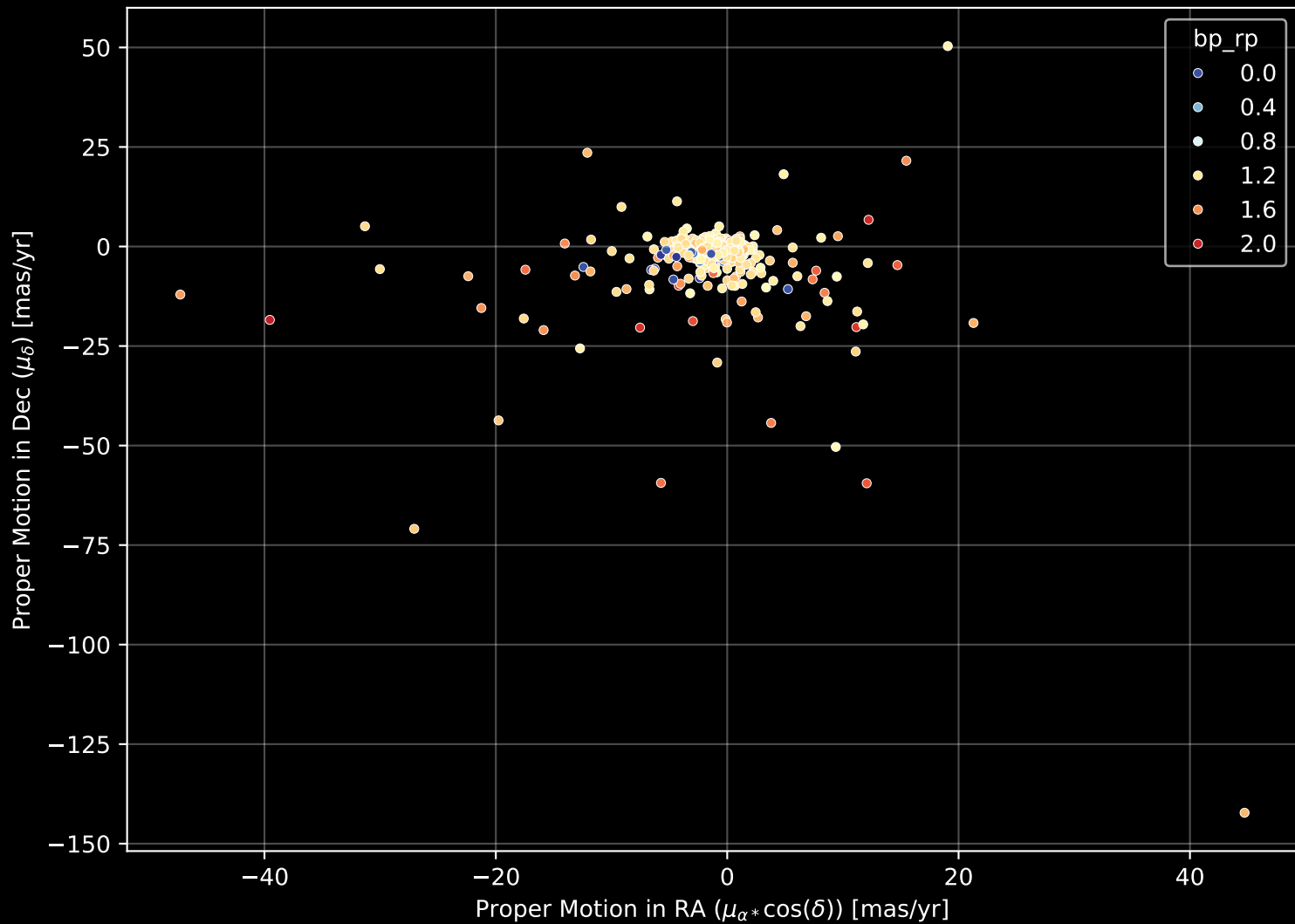
APOGEE DR17 Field: [210+08] Proper Motion Diagram (n= 512)
